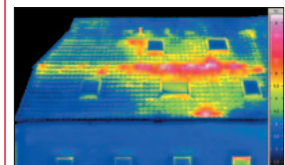
Insulation problem of a roof
